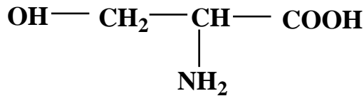
Serine
