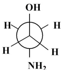
IY – Anti-form
