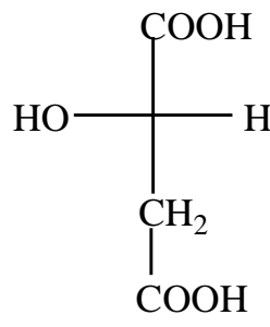
L-Malic Acid
