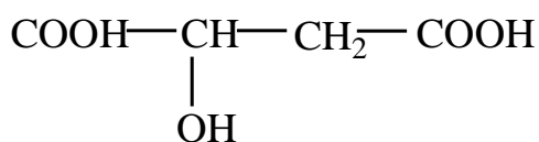
Malic acid
