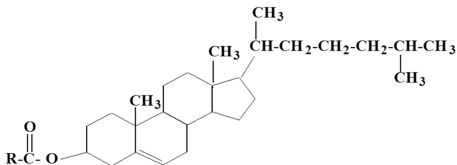
Figure 15.3 — General Formula for Cholesterol Esters
