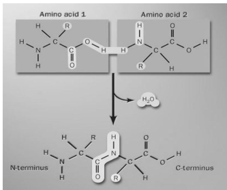
Figure 17.3 — The scheme of peptide bond formation
