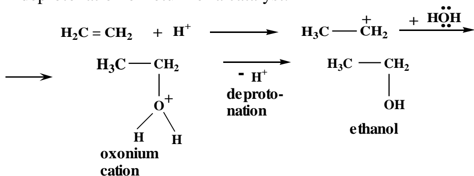
Figure 7.2 — The mechanism of ethene acid catalyzed hydration
