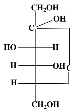
Cyclic formula for D-fructose
