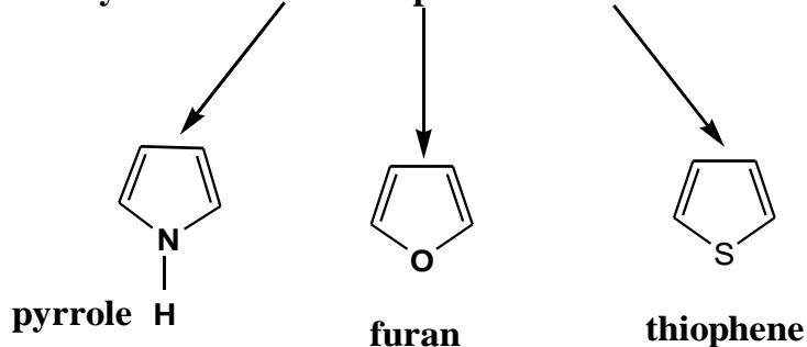
Figure 3.8 — Super Heteroaromatic systems with five-membered cycles
