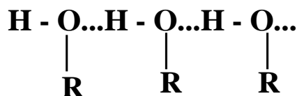
Association of alcohols molecules
