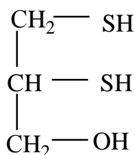
BAL
