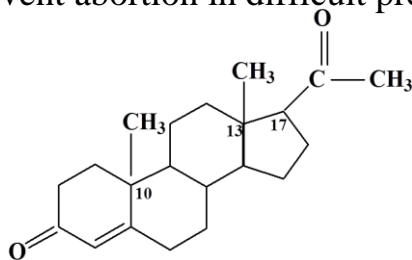
Figure15.11 — Progesterone
