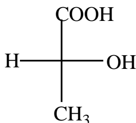
D-Lactic Acid
