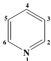
Pyridine
