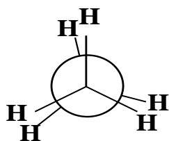
Eclipsed conformation (I)
