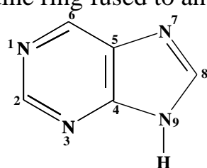
Purine
