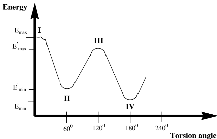
Figure 2.7 — Energy diagram for rotation colamine
