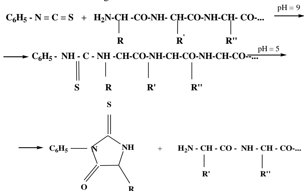
Phenylthiohydantoin derived from the N-terminal amino acid
