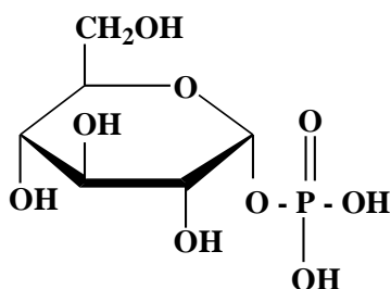
1-phosphate-D-glucopyranose
