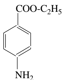
Anesthesine
