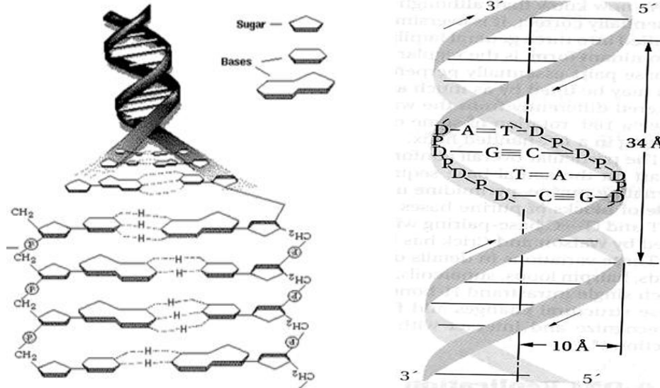
Figure 18.4 — Model and schematic representations of the DNA double helix The A—T pair is joined by two hydrogen bonds:
