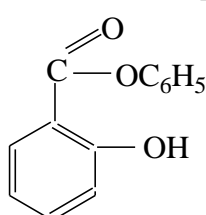
Phenyl salicylate
