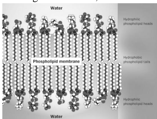
Figure 14.3 — The cell membranes of eukaryotic cells and some bacterial cells consist of three types of lipids — phospholipids, glycolipids and cholesterol molecules
