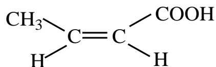
Isocrotonic acid
