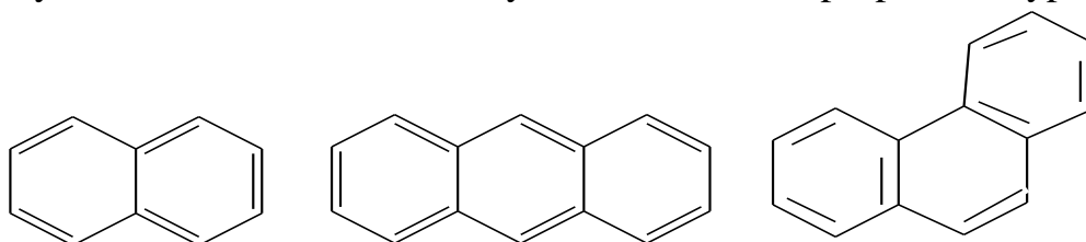
Naphthalene
