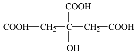
Citric acid
