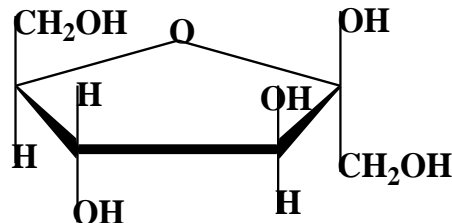
\beta -D- fructofuranose
