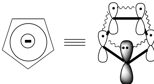
Figure 3.8 — p, \pi -Conjugated system of cyclopentadienyl
