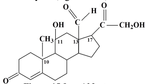
Figure 15.9 — Aldosterone
