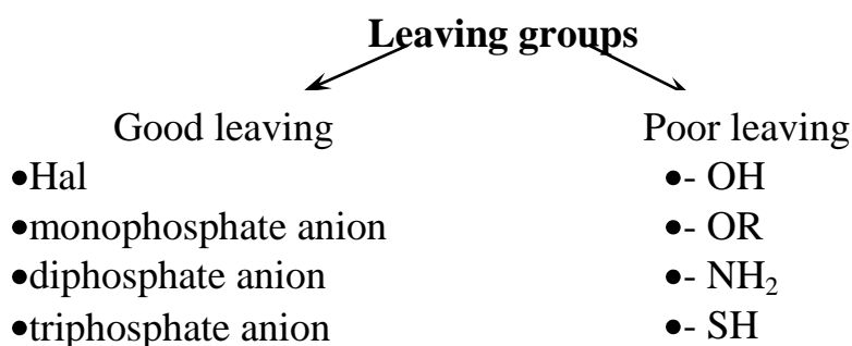
Figure 9.3 — Classification of leaving groups
