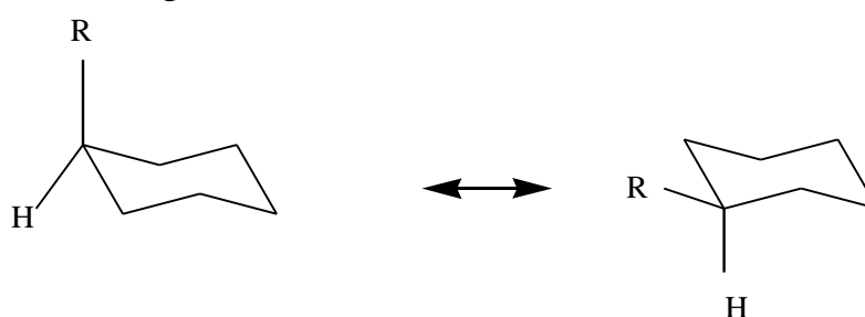
Figure 2.10 — Axial (R) or equatorial (H) positions
