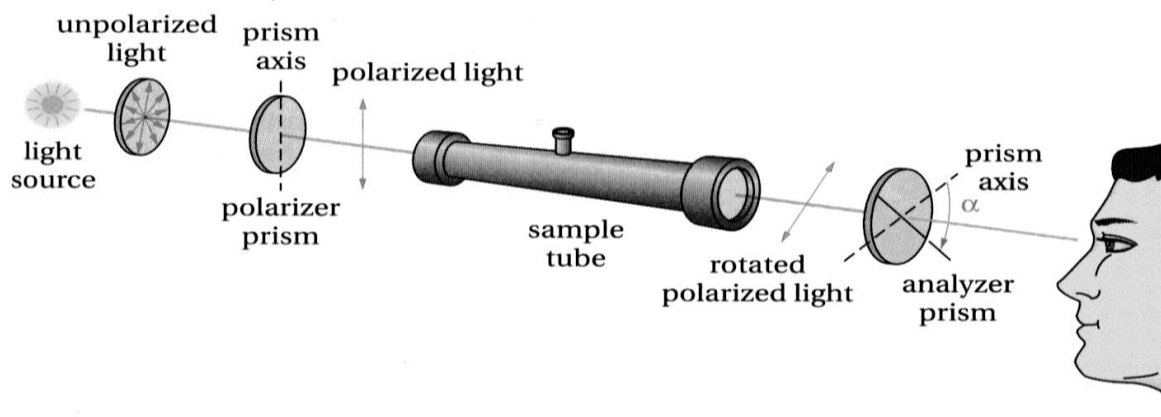
Figure 12.4 — Diagram of a polarimeter
