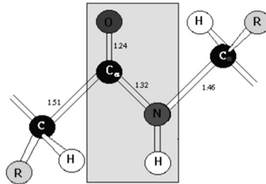
Figure 17.4 — The peptide group is planar with hydrogen of the substituted amino group is nearly always trans (opposite) to the oxygen of carbonyl group
