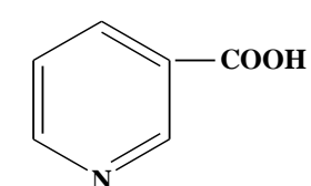
Nicotinic acid
