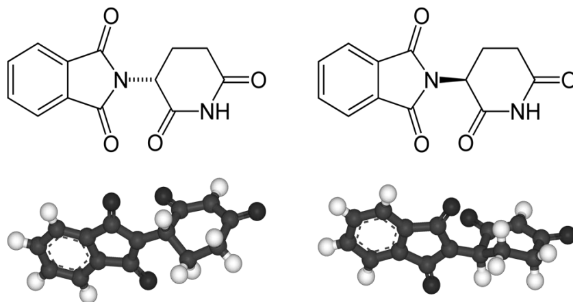
Figure 12.8 — Optical isomers of thalidomide
