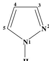
Pyrazole
