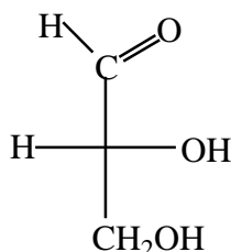
D-Glyceraldehyde
