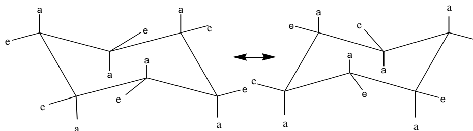
Figure 2.9 — Chair Inversion
