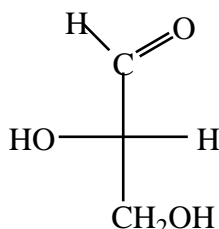
L-Glyceraldehyde
