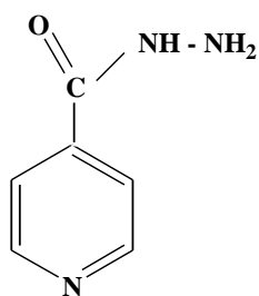
Isoniaside
