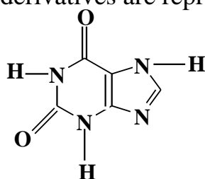
Xanthine (2, 6-dioxapurine)
