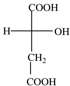
D-Malic Acid
