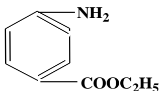
Anesthesine
