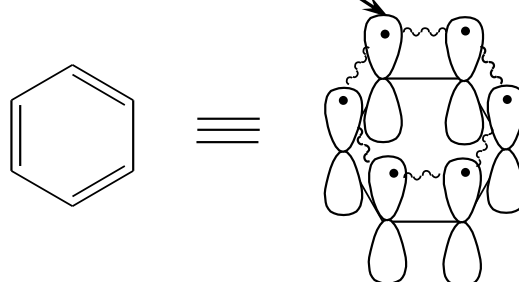
Figure 3.3 — \pi , \pi - Conjugated system of benzene
