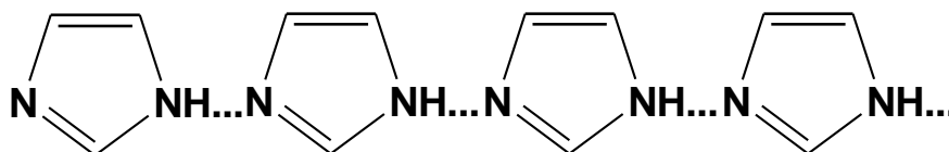
Association of imidazole molecules
