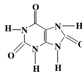
Uric acid (2, 6, 8-trioxapurine)
