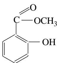
Methyl salicylate
