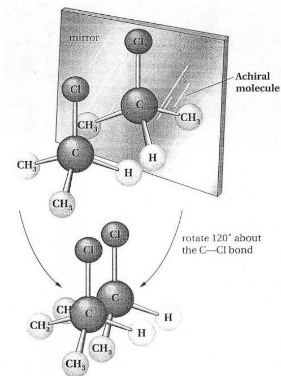
Figure 12.2 — Model of 2-chloropropane and its mirror image. The mirror image is super imposable on the original molecule
