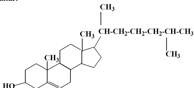
Figure 15.2 — Cholesterol
