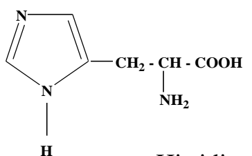
Histidine
