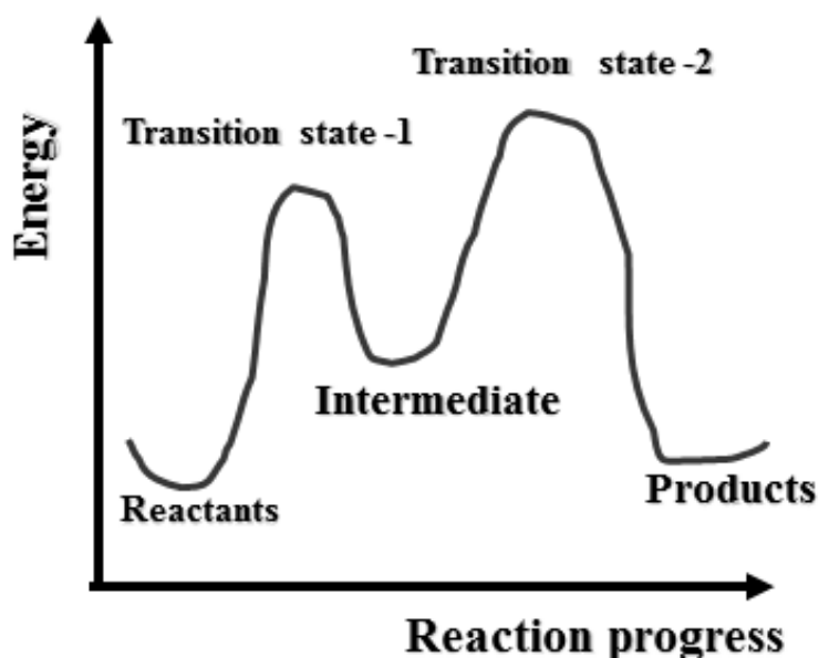
Figure 4.1 — Potential energy profile for stepwise reactions
