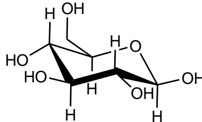
\beta -D-glucopyranose
