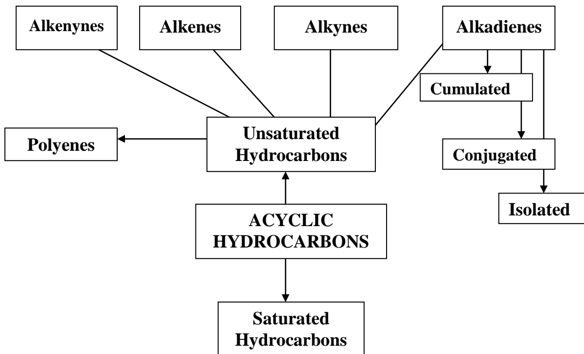
Figure 1.2 — Classification of acyclic compounds
