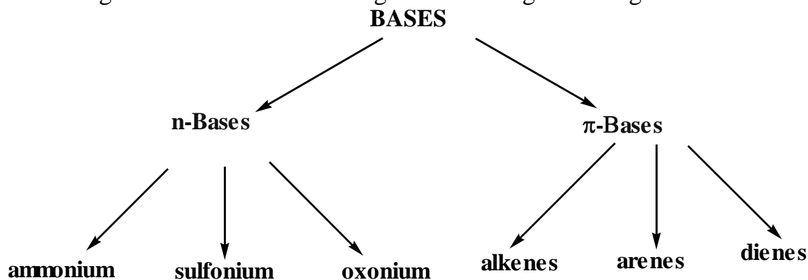
Figure 5.2 — Types of organic bases
