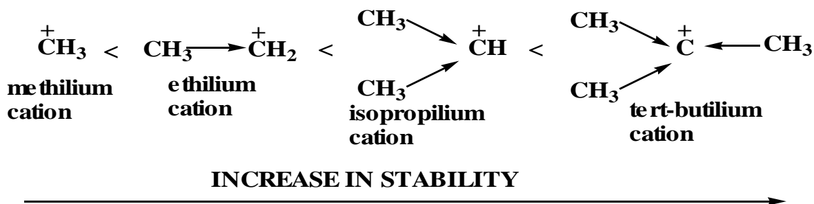
Figure 4.2 — Stability of carbocations
