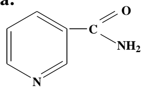
Nicotinamide
