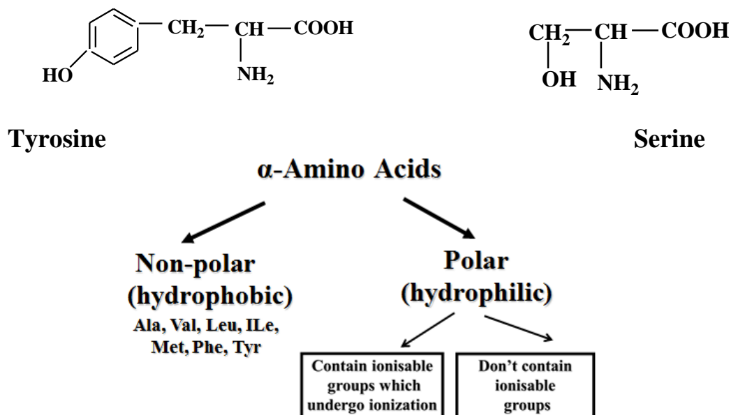
Figure 17.2 — Classification of \alpha -amino acids according to polarity of their radicals
