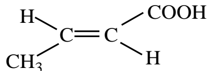
Crotonic acid
