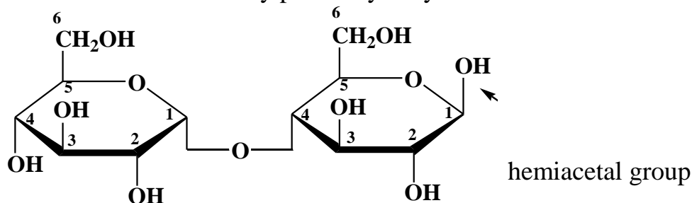
\alpha -D-glucopyranosyl-(1 \rightarrow 4)- \beta -D-glucopyranose
