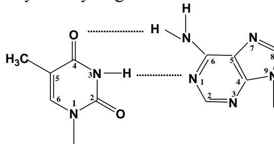
Figure 18.4 — Model and schematic representations of the DNA double helix The A—T pair is joined by two hydrogen bonds:
