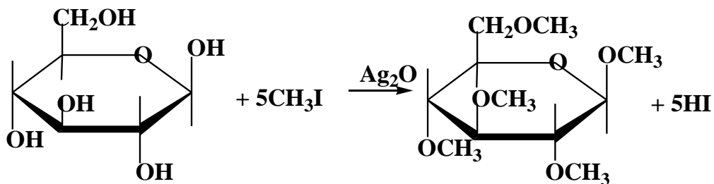
O-methyl-2,3,4,6-tetramethyl- \beta -D-glycopyranoside
