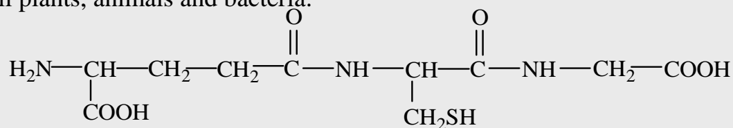
\gamma -Glu-Cys-Gly
