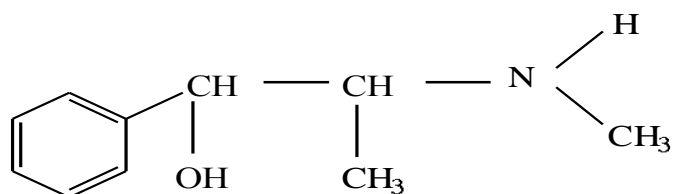
Ephedrine
