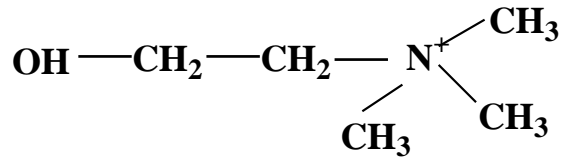
Choline
