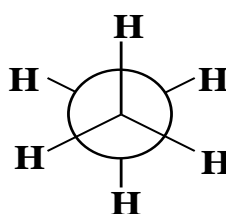
Staggered conformation (II)
