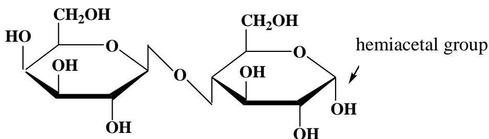
\beta -D-galactopyranosyl-(1 \rightarrow 4)- \alpha -D-glucopyranose
