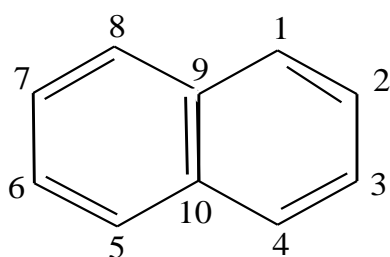
naphthalene
