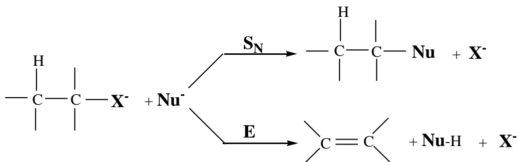
Figure 9.2 — Nucleophilic substitution and elimination in competition
