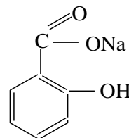
Sodium salicylate
