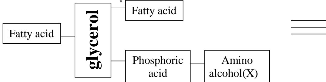
Serine
