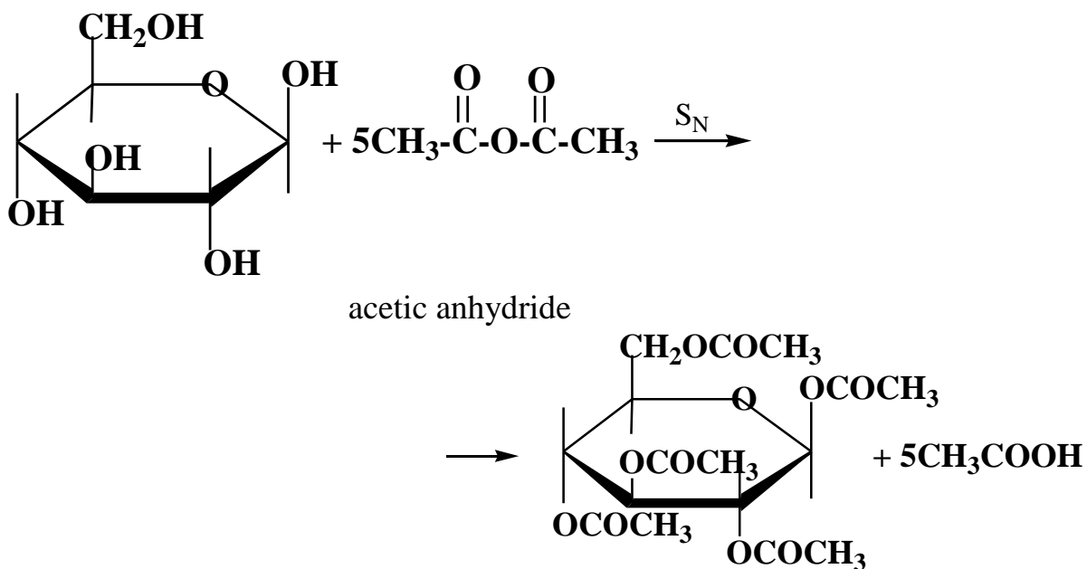
\beta -D-glycopyranoside pentaacetate
