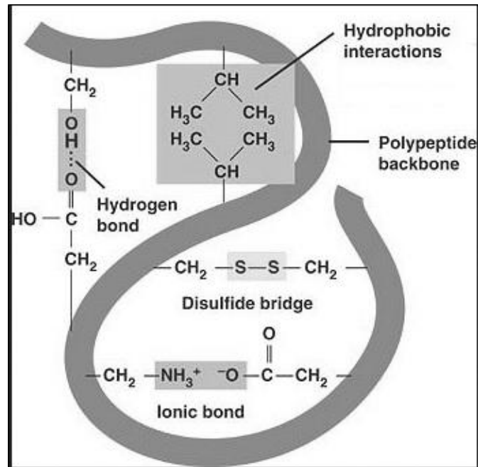
Figure 17.8 — Tertiary structure of proteins
