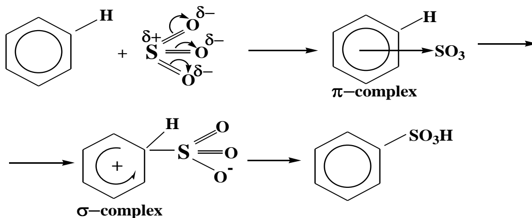
Figure 8.1 — Distribution of electron density in sulfur trioxide molecule
