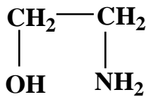
Ethanolamine (Calamine)
