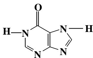
Hypoxanthine (6-oxapurine)
