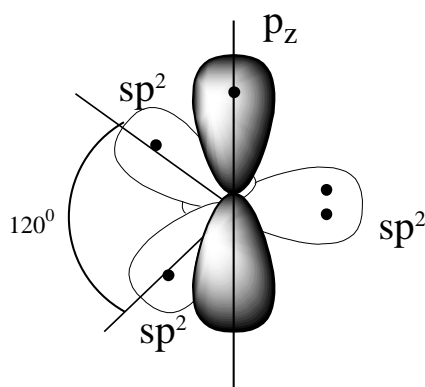
Figure 3.5 — Electron structure of pyridine nitrogen
