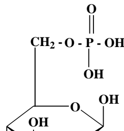
1,6-diphosphate-D-fructofuranose (Phosphate Ester of Fructose)
