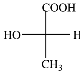
L-Lactic acid
