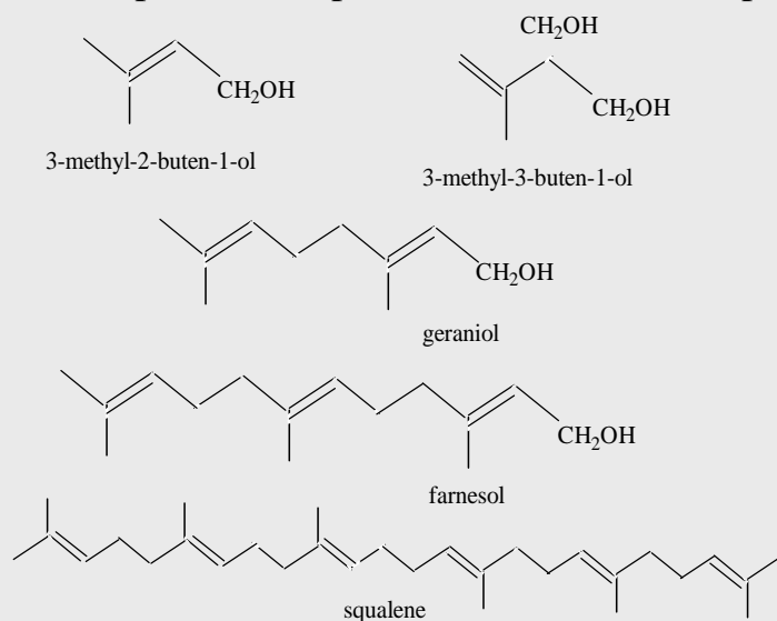
Figure 5.1— Biologically important alcohols and phenols
