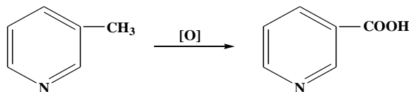
\beta -Picoline
