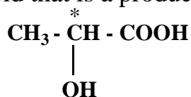
Figure 12.6 — Glyceraldehyde and their enantiomers
